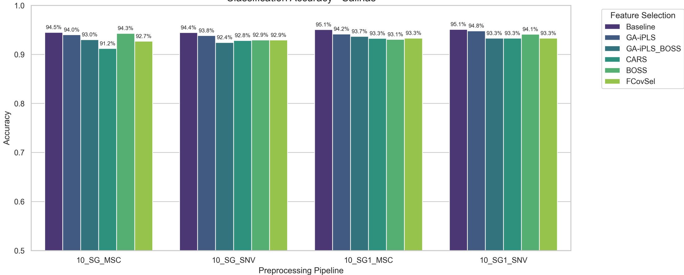
Classification Accuracy - Salinas
